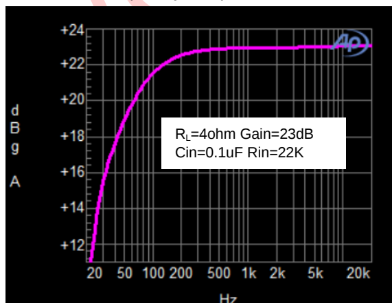
Frequency Response
