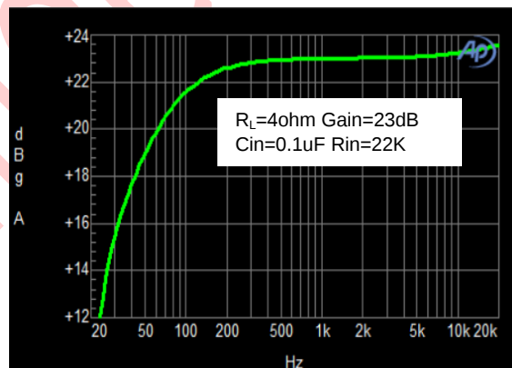
Frequency Response
